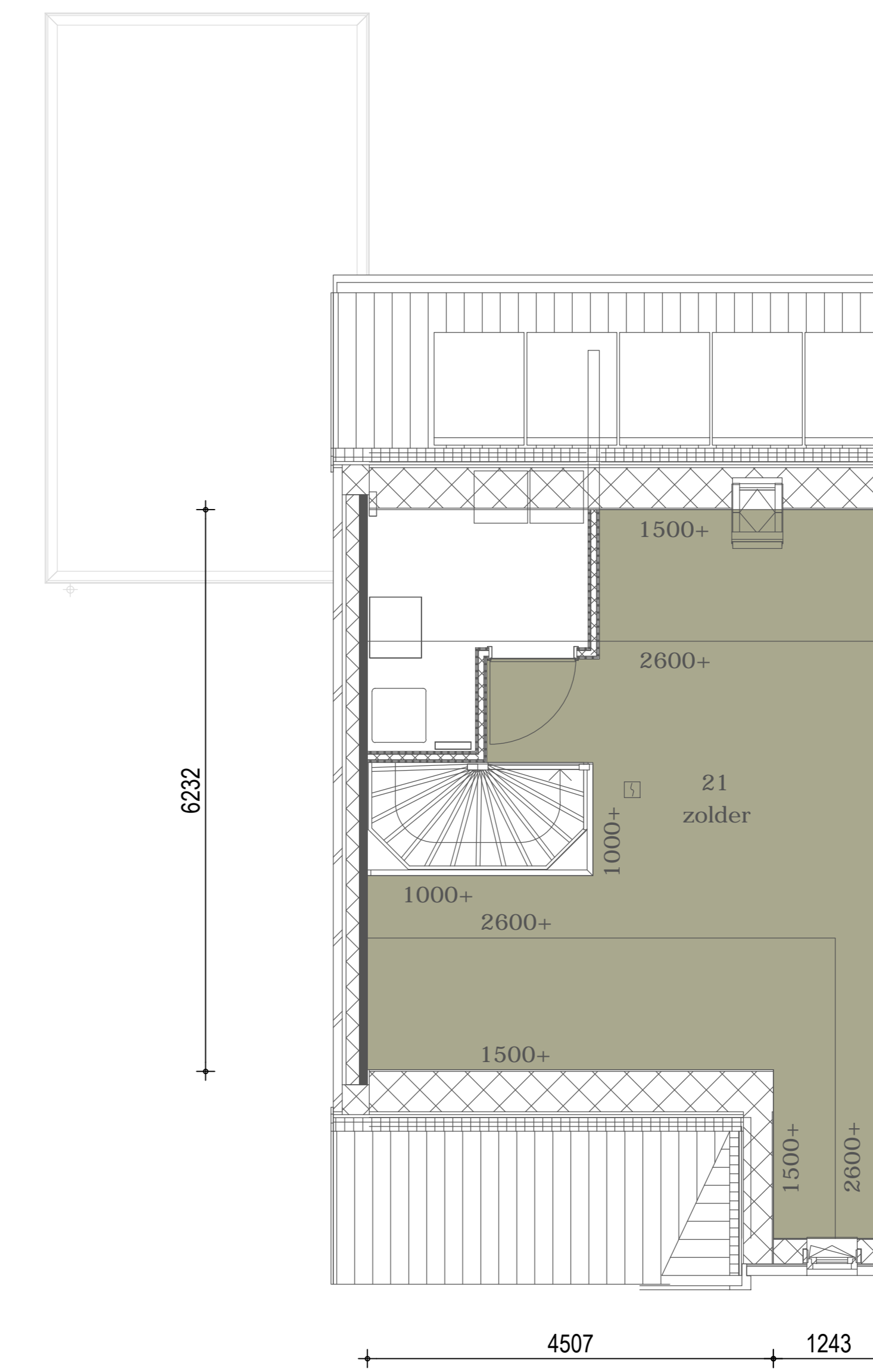
Zolder
